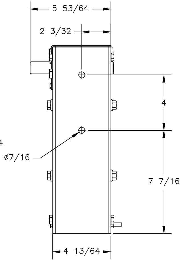
SIDE VIEW (MOUNTING HOLE PATTERN SAME ON BOTH SIDES)
